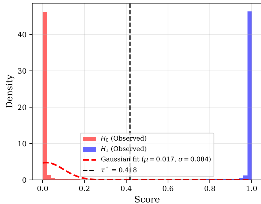
DNN-2feat
